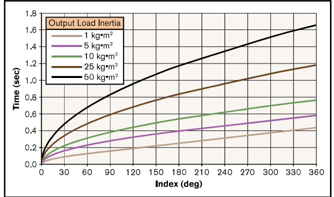
CRD350P-MR (MRS, MRG, MRO) Timing Diagram
