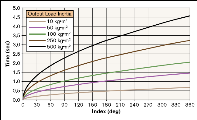
CRD350P-PL Timing Diagram*
