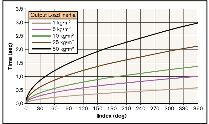
CRD350N-MR (MRS, MRG, MRO) Timing Diagram
