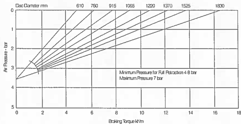
Brake performance at 19.5 kN braking force
