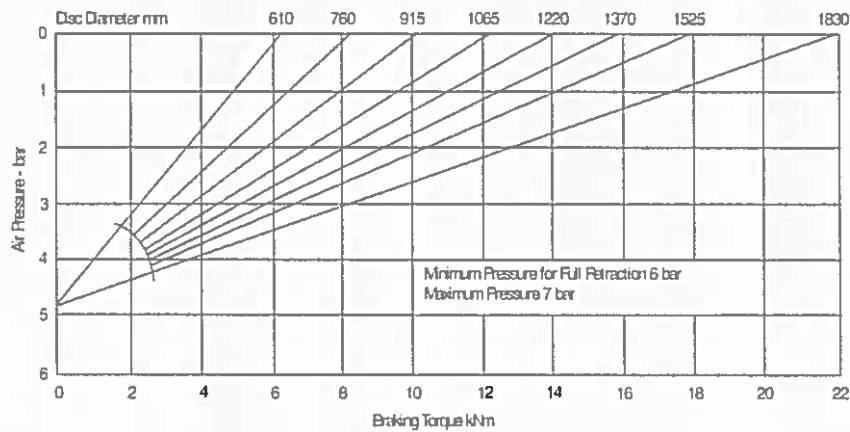
Brake performance at 25 kN braking force
