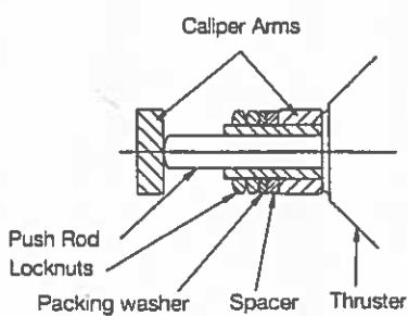
Fig 1. Assembly for 8mm disc
