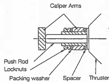
Fig 2. Assembly for 12.7mm disc
