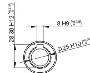
Input shaft detail Scale 1:2 (both sides)
